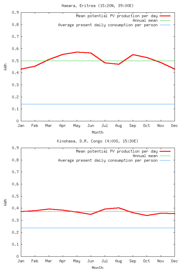
Figure 3: Seasonal variation of the daily PV electricity generation from a 100 \text{ W}_p system in Asmara and Kinshasa (red line). The graphs also show the annual mean daily generation (green line) and this is compared with the average daily electricity consumption per capita in the respective countries (blue line, source [12]).
