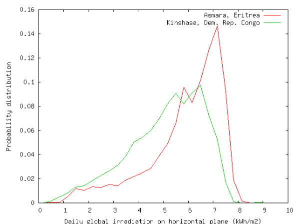
Figure 4: Average probability distribution of daily irradiation ( \text{kWh m}^{-2} ) within a year in Asmara and Kinshasa. The data represent the period 1985-2004.
