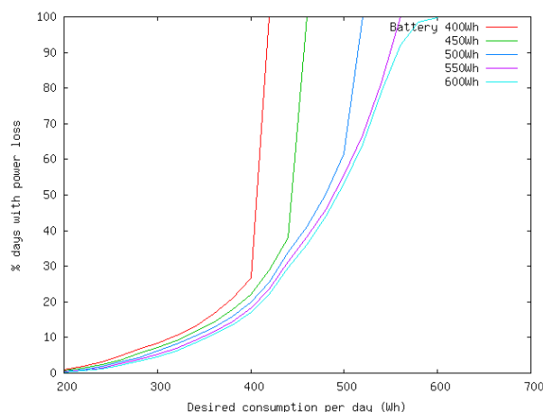
Figure 5: Performance of a 100 W p system in Asmara, depending on desired power consumption and battery size, indicated by the percentage of days where power runs out. Calculation is based on daily irradiation data for the period 1985-2004.
